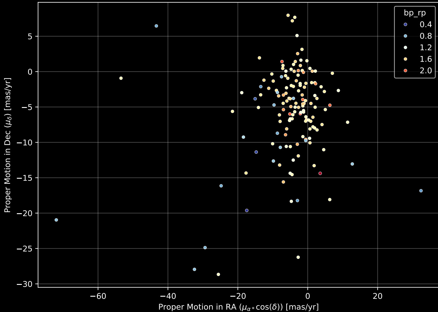
APOGEE DR17 Field: [000+30] Proper Motion Diagram (n= 147)
