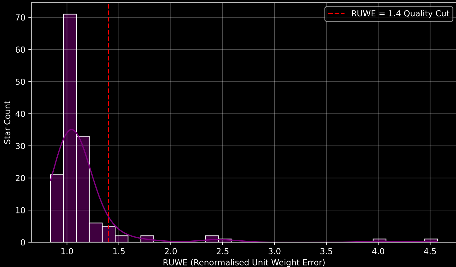
GAPOGEE DR17 Field [000+30] RUWE Distribution (n= 145)
