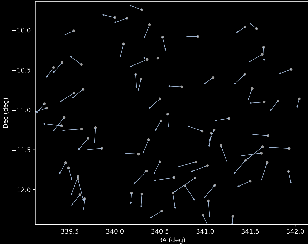
APOGEE DR17 Cluster 1 Proper Motion Vectors (n=76)
