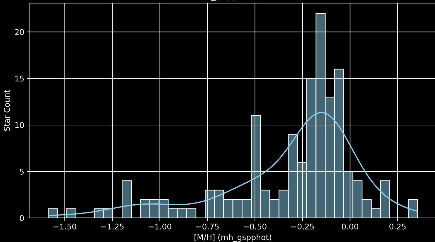
APOGEE DR17 Field: [000+30 [M/H] (mh_gspphot) (n= 147)
