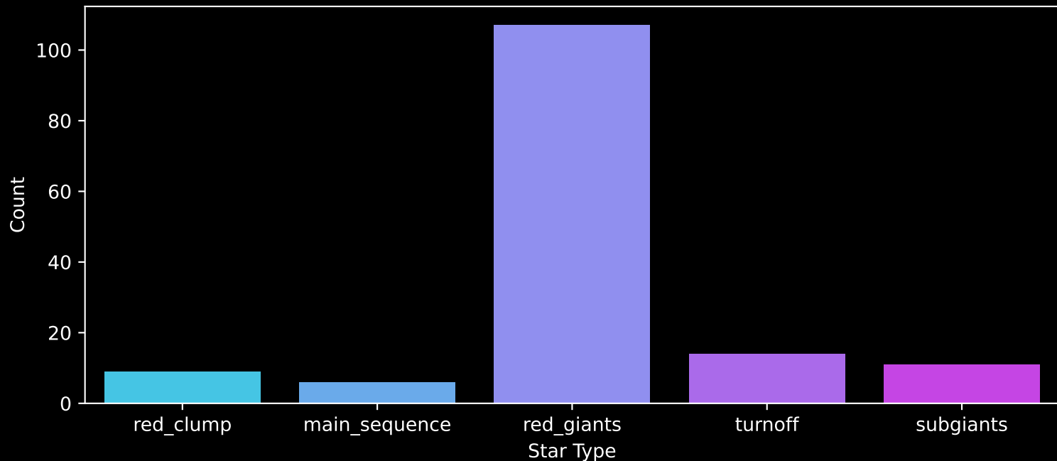
APOGEE DR17 Field: [000+30] Count plot of Star Type
