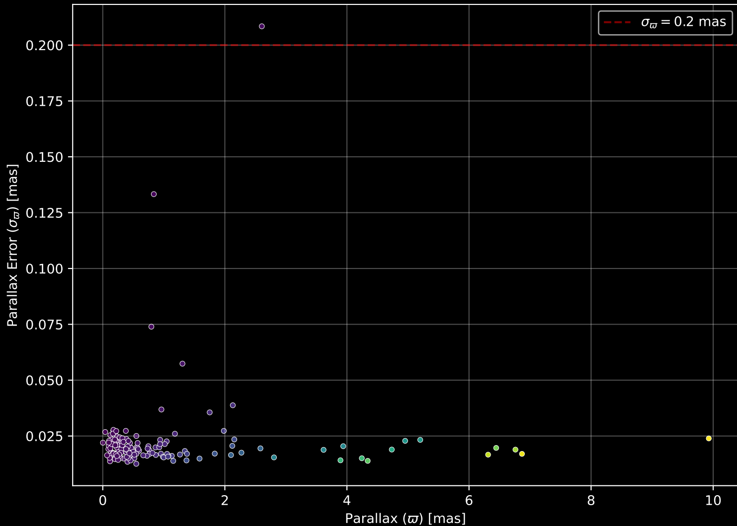
APOGEE DR17 Field: [000+30] Parallax Quality (n= 147)
